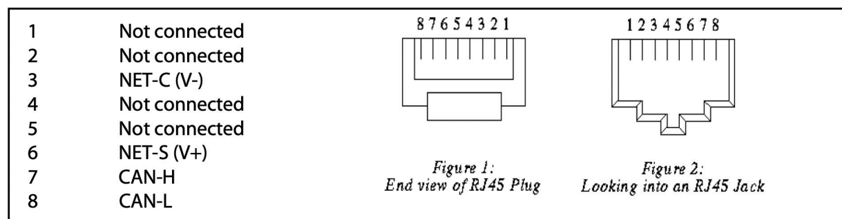
Victron VE.Can-pinout
